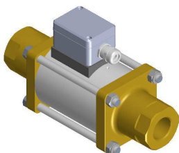
Klemmkasten terminal box Schutzart: IP 65 protection class: IP 65 PG11-Verschraubung PG11-fitting elektrische Option = 29 electrical option = 29
