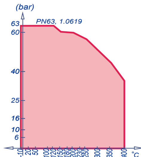
P/T Type YVMN8/YVSN8 (1/2" ~ 1") PN63 (1.0619)
